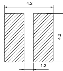
Recommended PC Board Pattern
